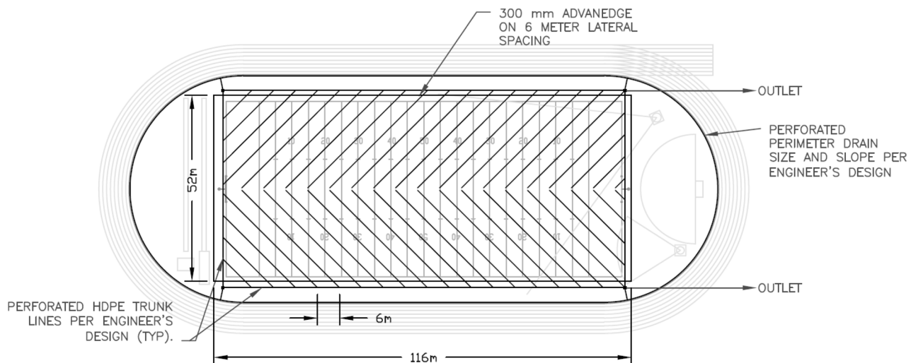
Figure 2: Typical Synthetic Turf Herringbone Drainage Layout
