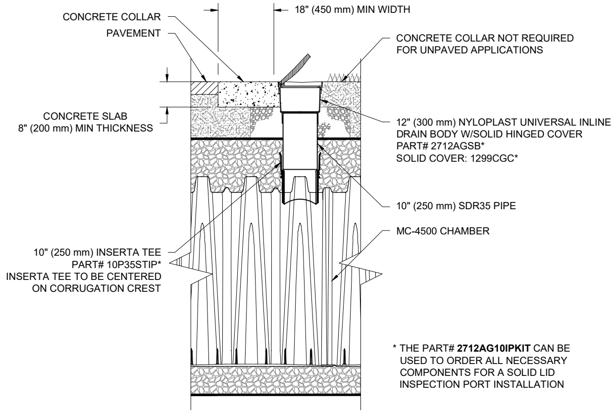
MC-4500 10" (250 mm) INSPECTION PORT DETAIL
