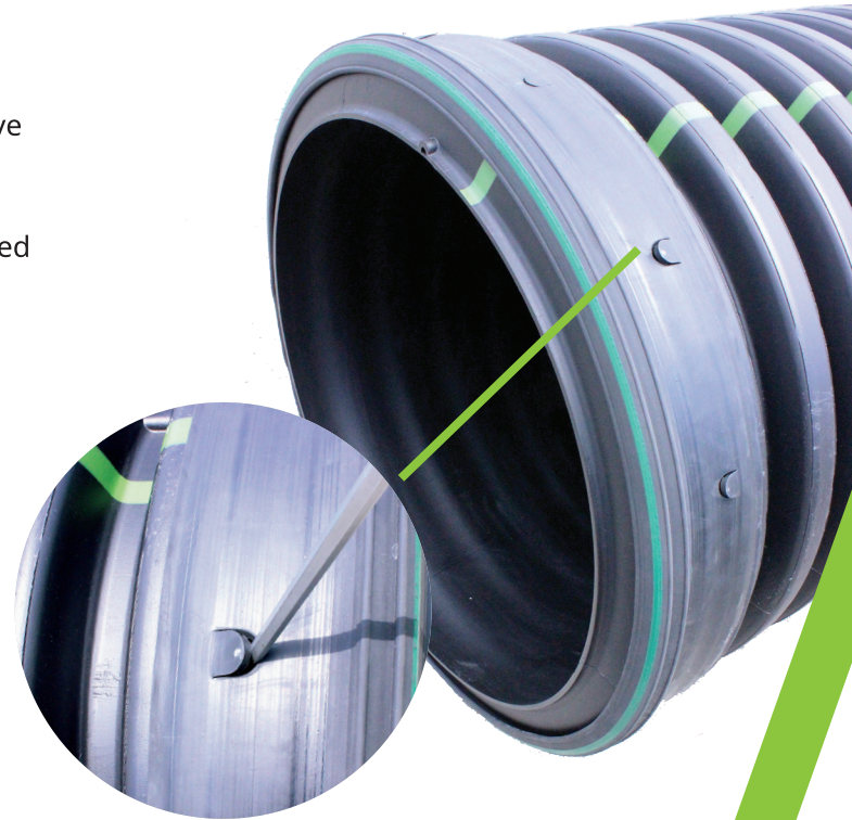
Pictured above is a 24"-36" (600-900 mm) saddle gasket.
