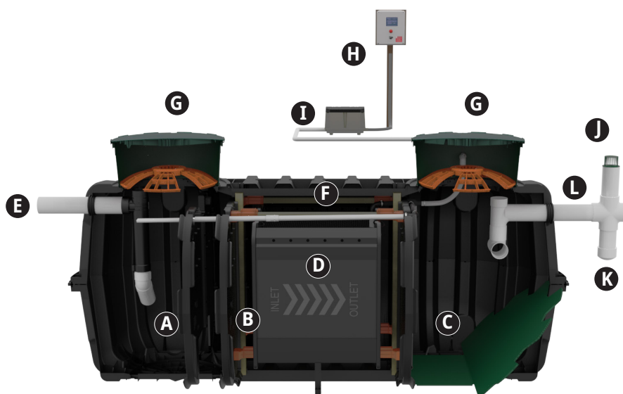
ECOPOD Edge500 installed in the Infiltrator CM-1060 tank
