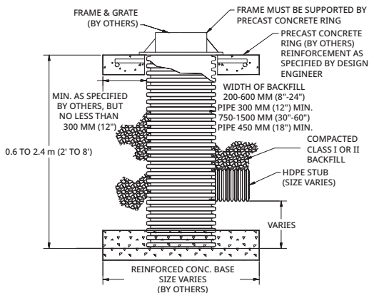
Figure 6: Vertical Riser
