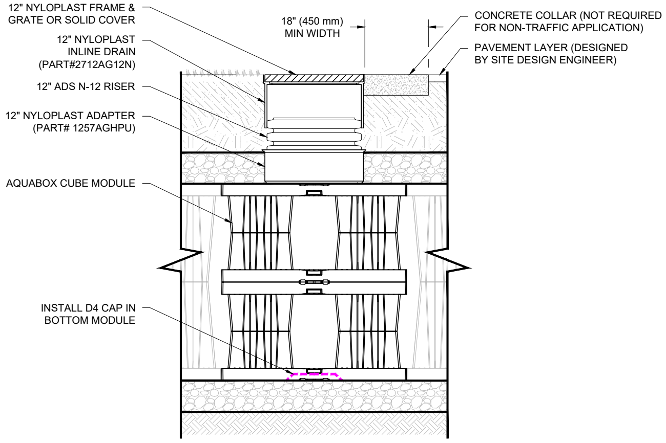
AQUABOX INSPECTION PORT DETAIL NTS
