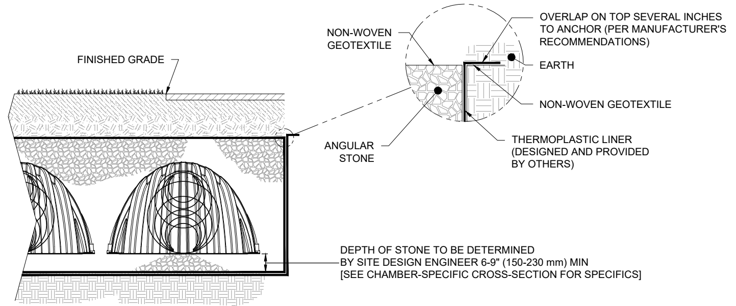
MEMBRANE LINER DETAIL NTS
