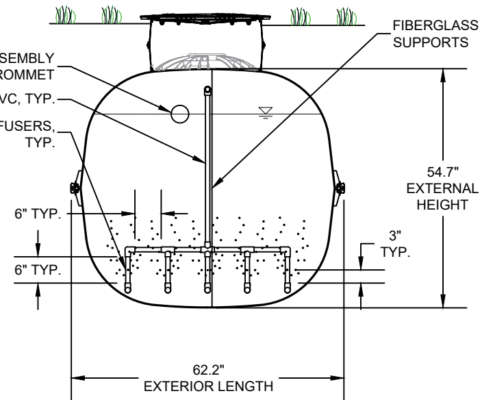
SIDE VIEW SECTION A-A
