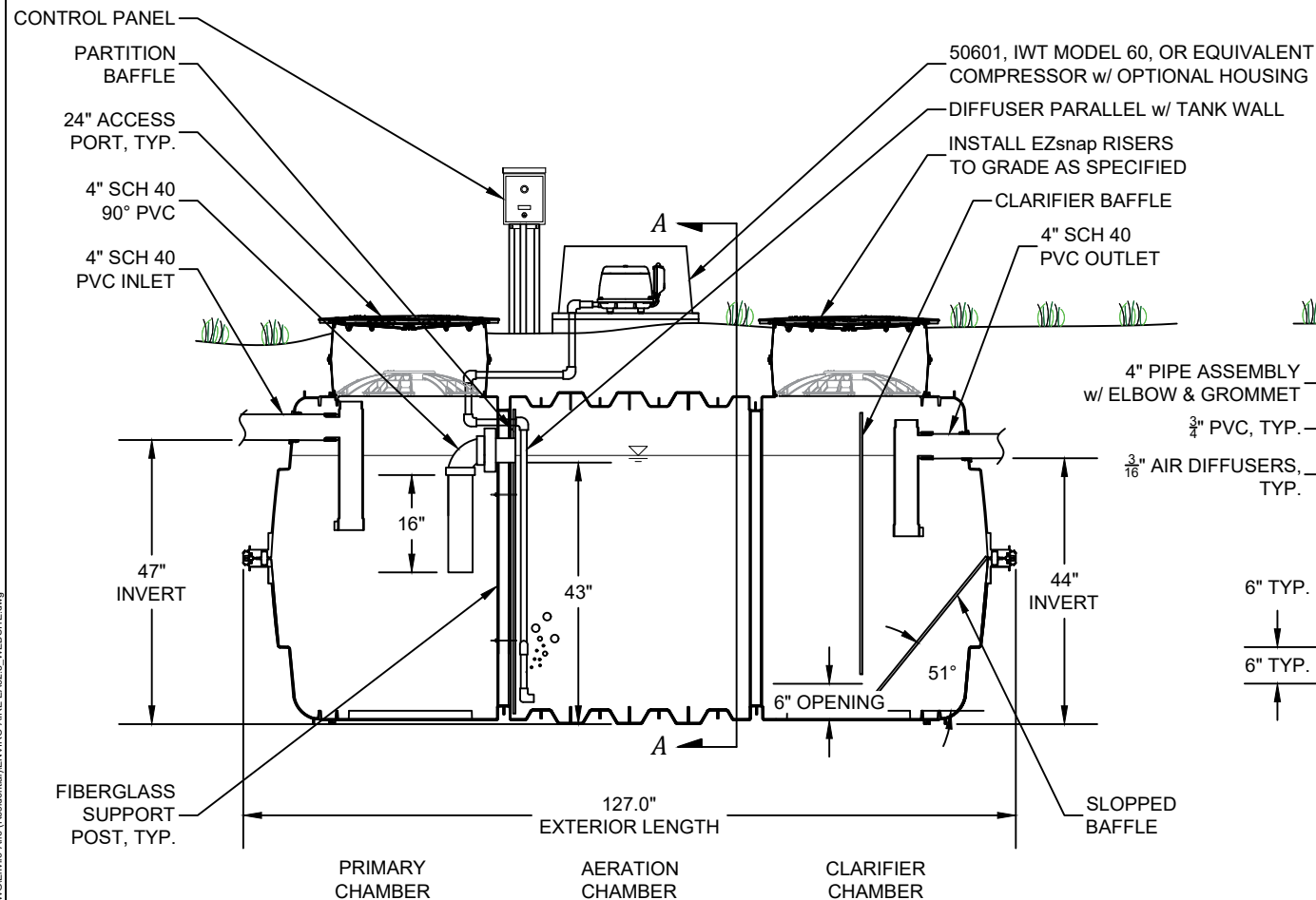
ELEVATION VIEW
