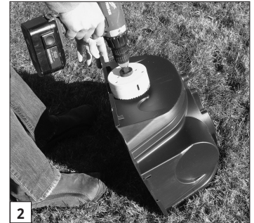
Drill endcap on end.
