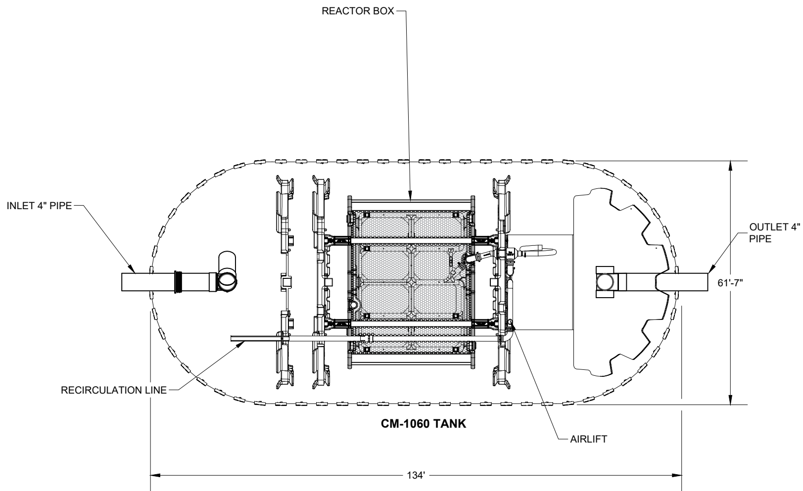
PLAN VIEW
