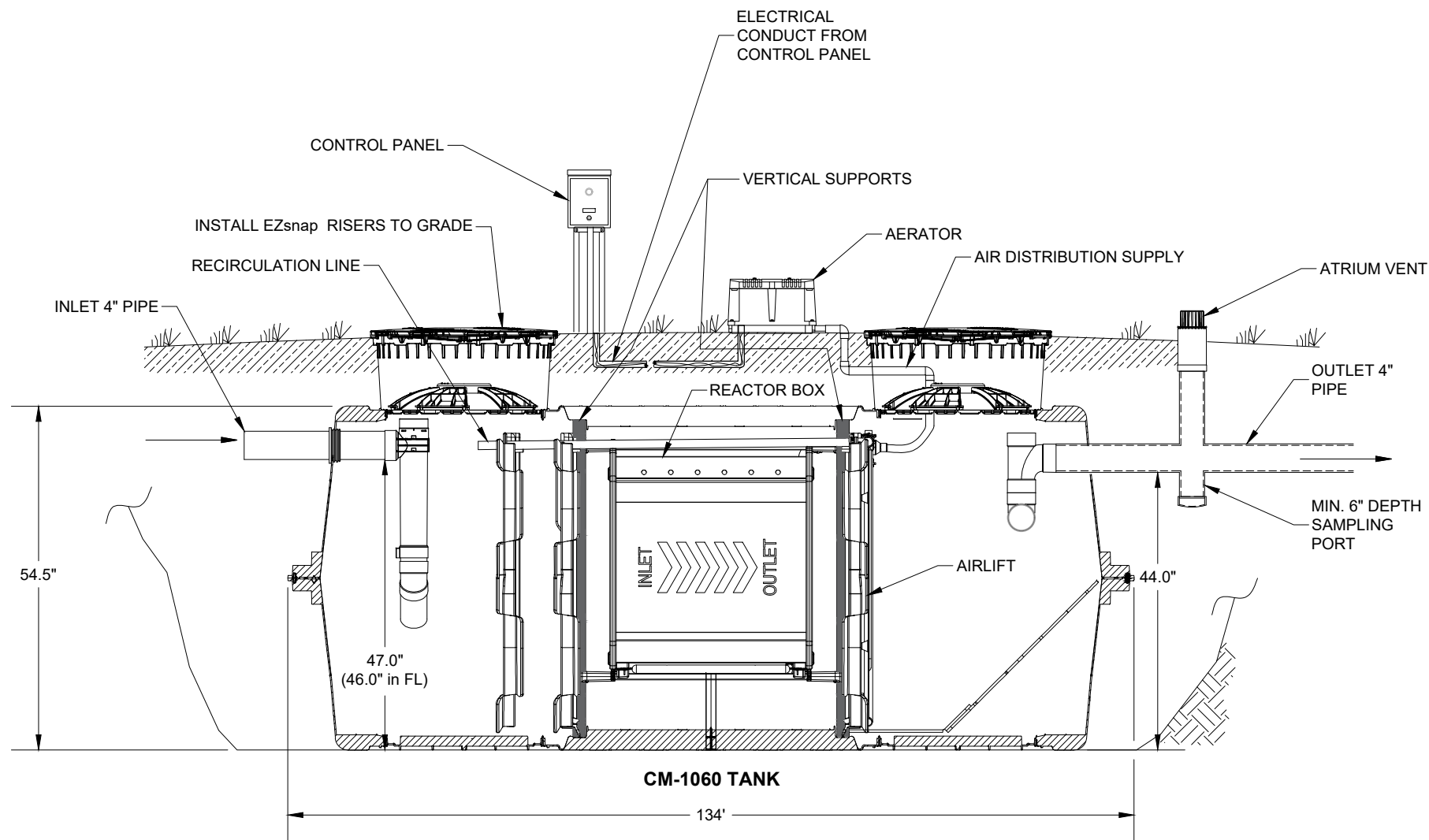
CROSS SECTION
