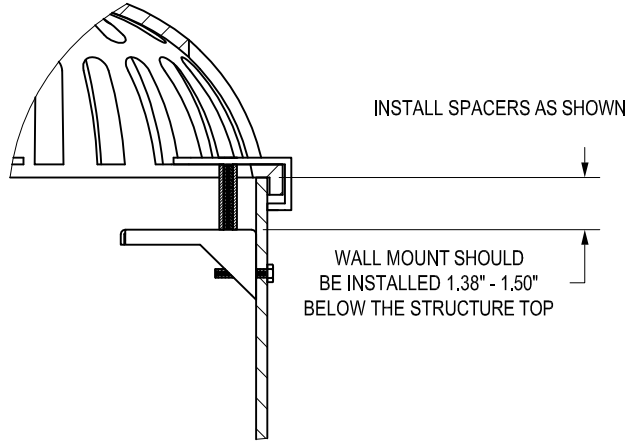
CUTOUT DETAIL
