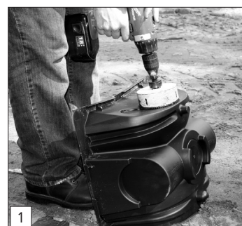
Drill endcap.
