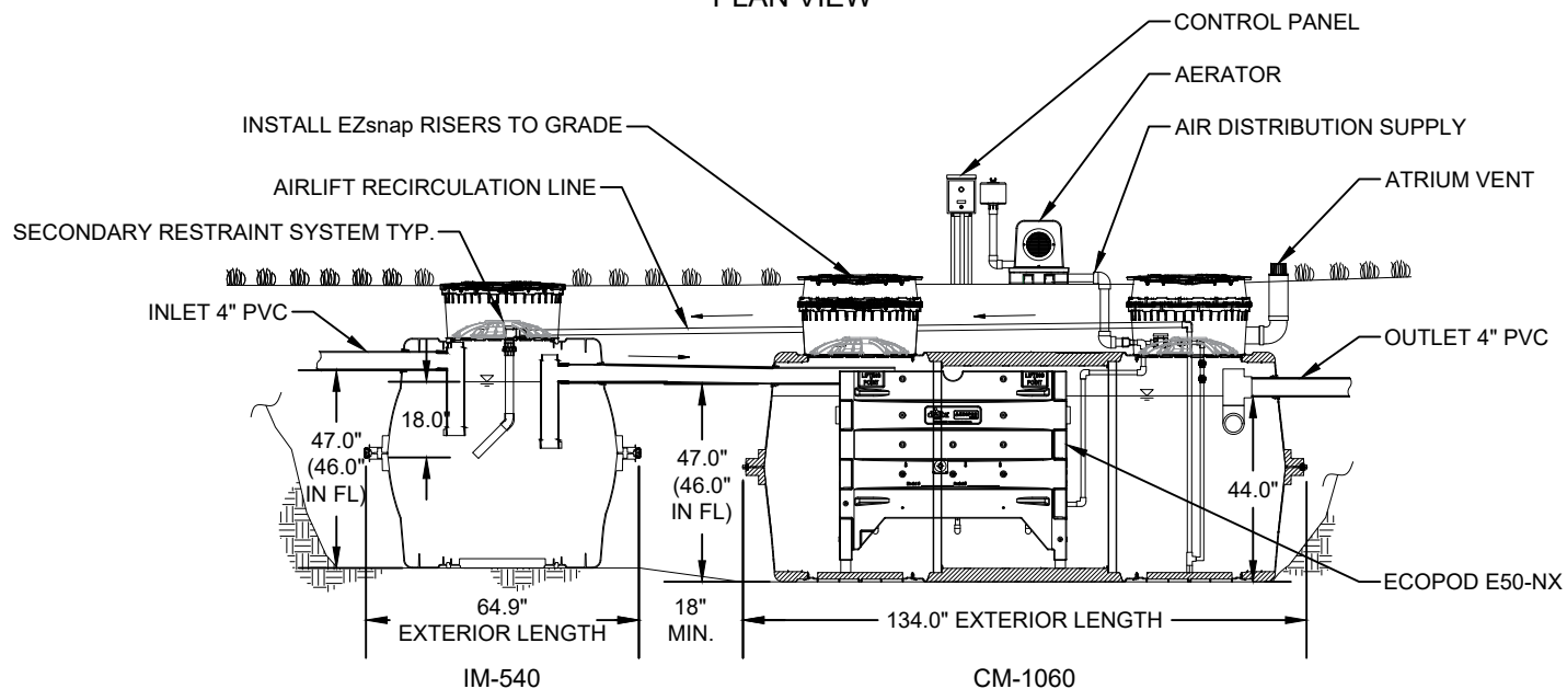
SECTION VIEW
